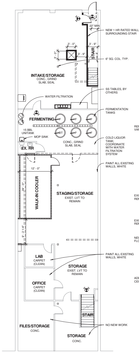
1 BASEMENT 1/8" = 1'-0"
