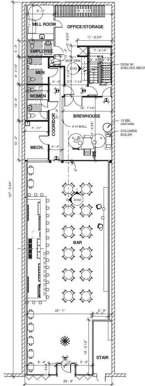
3 FIRST FLOOR 1/8" = 1'-0"
